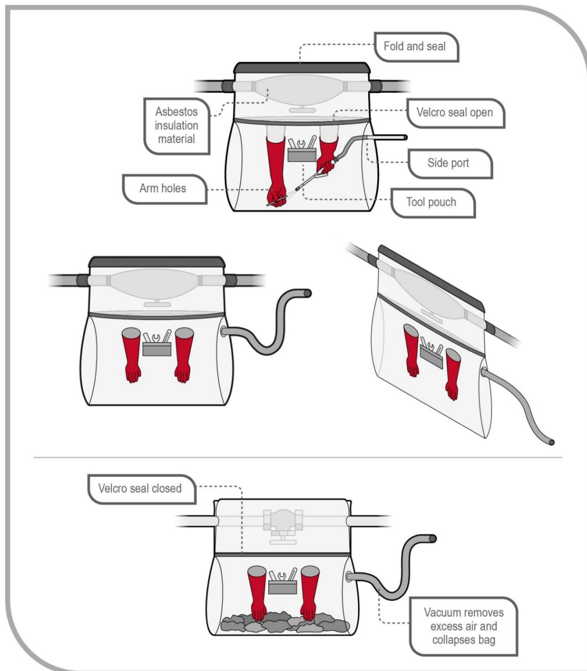
Figure 8 Using a glove bag
