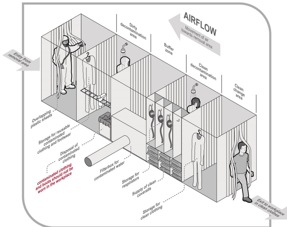
Figure 4 Decontamination unit
