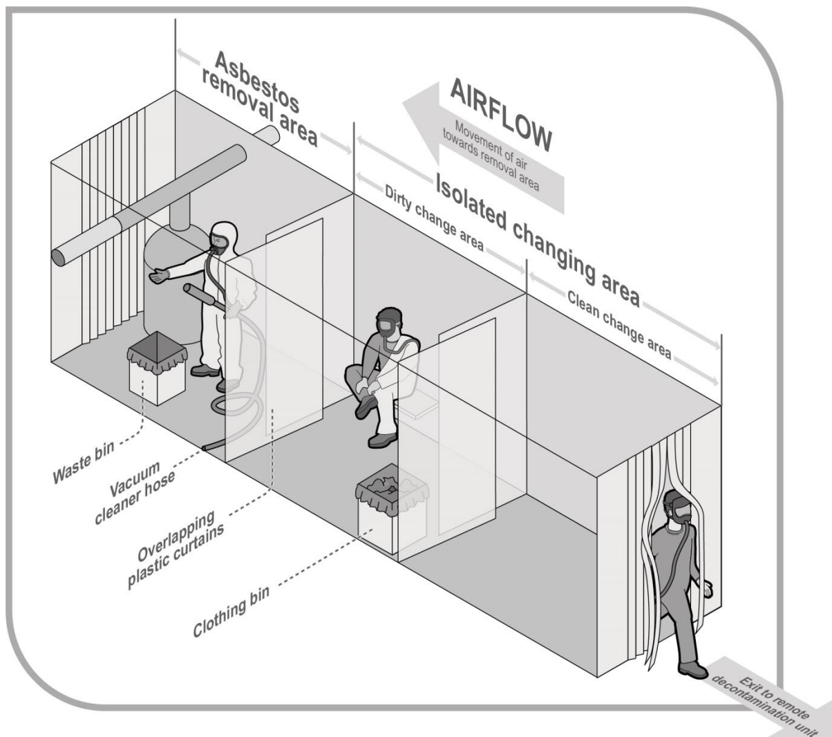
Figure 5 Preliminary decontamination procedure where a remote decontamination unit is used
