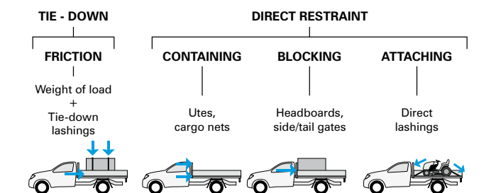
Figure 1. Restraint Methods
